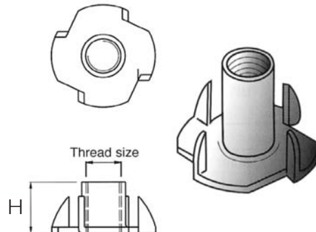
H = 11 mm for the 4090 H = 8.5mm for the 4093
